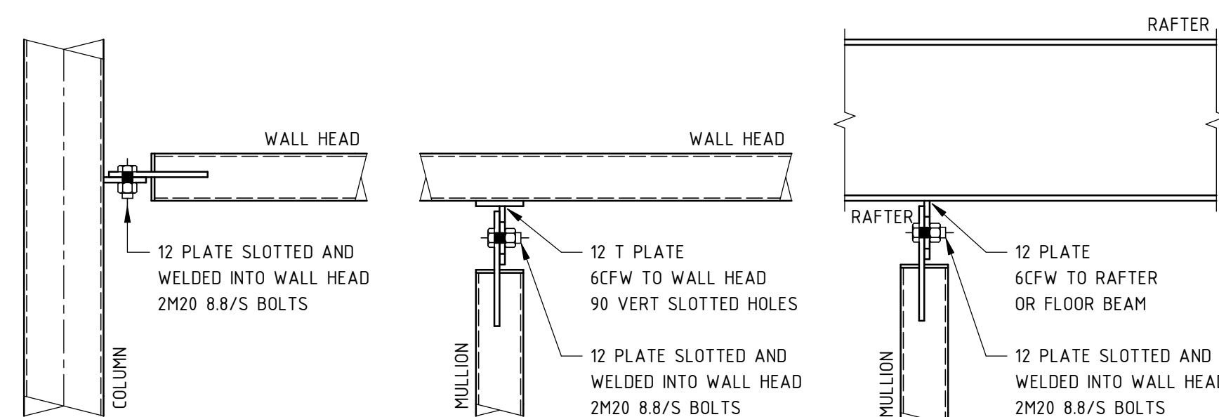
TYPICAL WALL HEAD AND MULLION CONNECTION DETAILS
