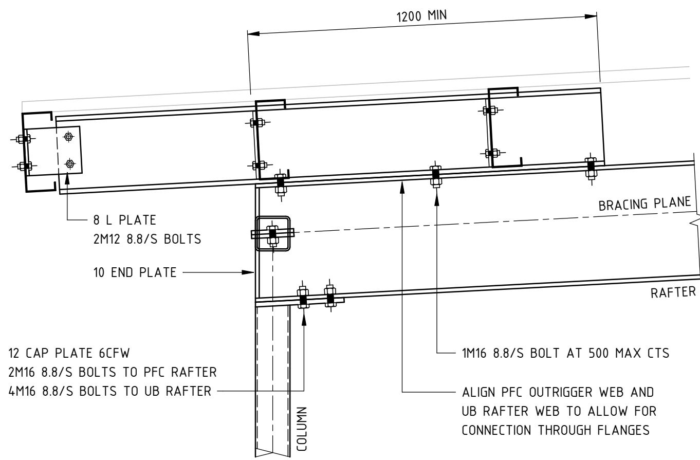
TYPICAL OFFICE COLUMN TO RAFTER DETAIL
