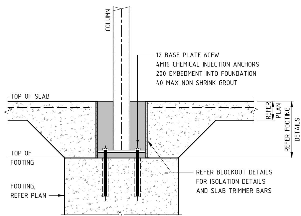
TYPICAL OFFICE COLUMN BASE PLATE DETAIL
