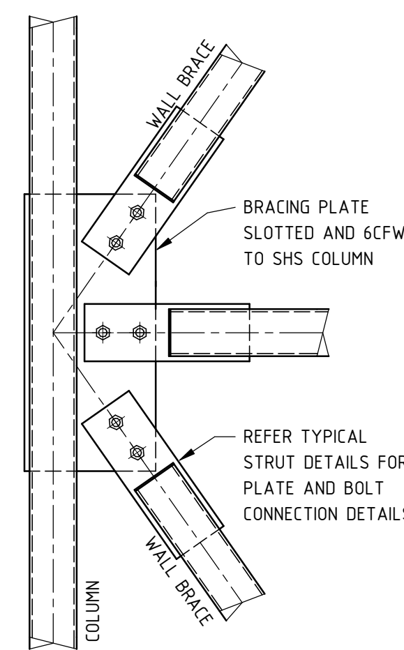
TYPICAL OFFICE WALL BRACE DETAIL
