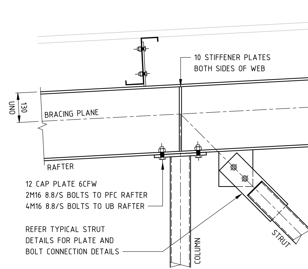
TYPICAL OFFICE COLUMN TO RAFTER DETAIL
