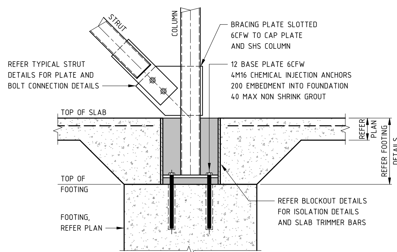
TYPICAL OFFICE COLUMN BASE PLATE DETAIL AT WALL BRACING
