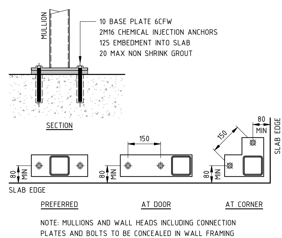
TYPICAL OFFICE MULLION BASE PLATE TO SLAB DETAILS
