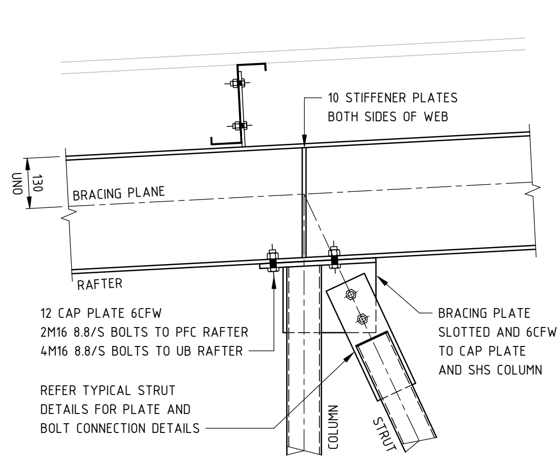
TYPICAL OFFICE COLUMN TO RAFTER DETAIL
